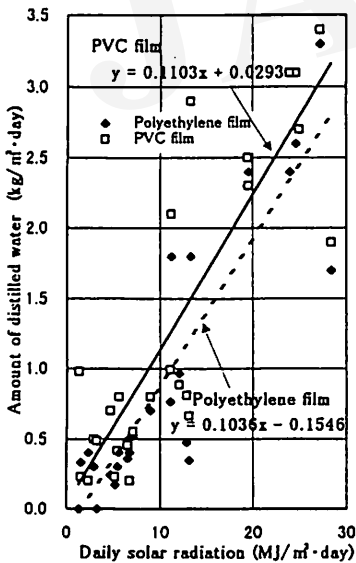
Fig.5 Radiations between daily solar radiation and amount distilled water (in case of non-fan)
