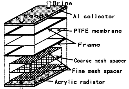
Fig. 2 A schematic diagram of the module
