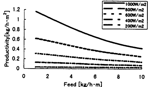
Fig.5-(b) Productivity of Simulation in case of Downward Feed
